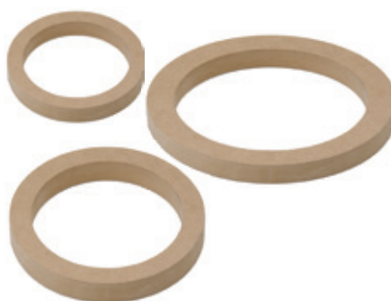
MDF SPEAKER RINGS SR5 4 3/4" INSIDE, 6" OUTSIDE PAIR SR6 5 7/16" INSIDE, 7" OUTSIDE PAIR SR8 7" OUTSIDE, 8.5" OUTSIDE PAIR SR10 9 1/8" INSIDE, 11" OUTSIDE EA SR12 11 1/8" INSIDE, 13" OUTSIDE EA SR15 13 7/8" INSIDE, 15 7/8" OUTSIDE EA
